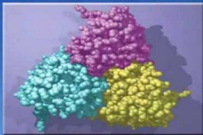
Protein Structure
