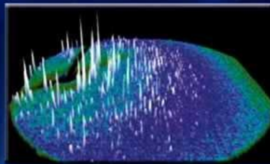
Diffraction Pattern
